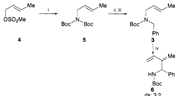
Scheme 3 Reagents and conditions: i, Boc 2 NH, K 2 CO 3 , LiI, butanone, 80 °C, 14 h, 65%; ii, TFA, CH 2 Cl 2 , 14 h; iii, KH, BnCl, 0 °C to room temp. 14 h, 92%; iv, Bu n Li, Et 2 O-HMPA (4 : 1), -78 to -40 °C, 14 h, 82%
